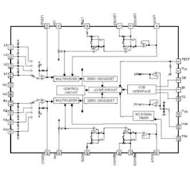
IC312: 313 LCT334M Single-Chip Electronic Volume and Tone Control System
