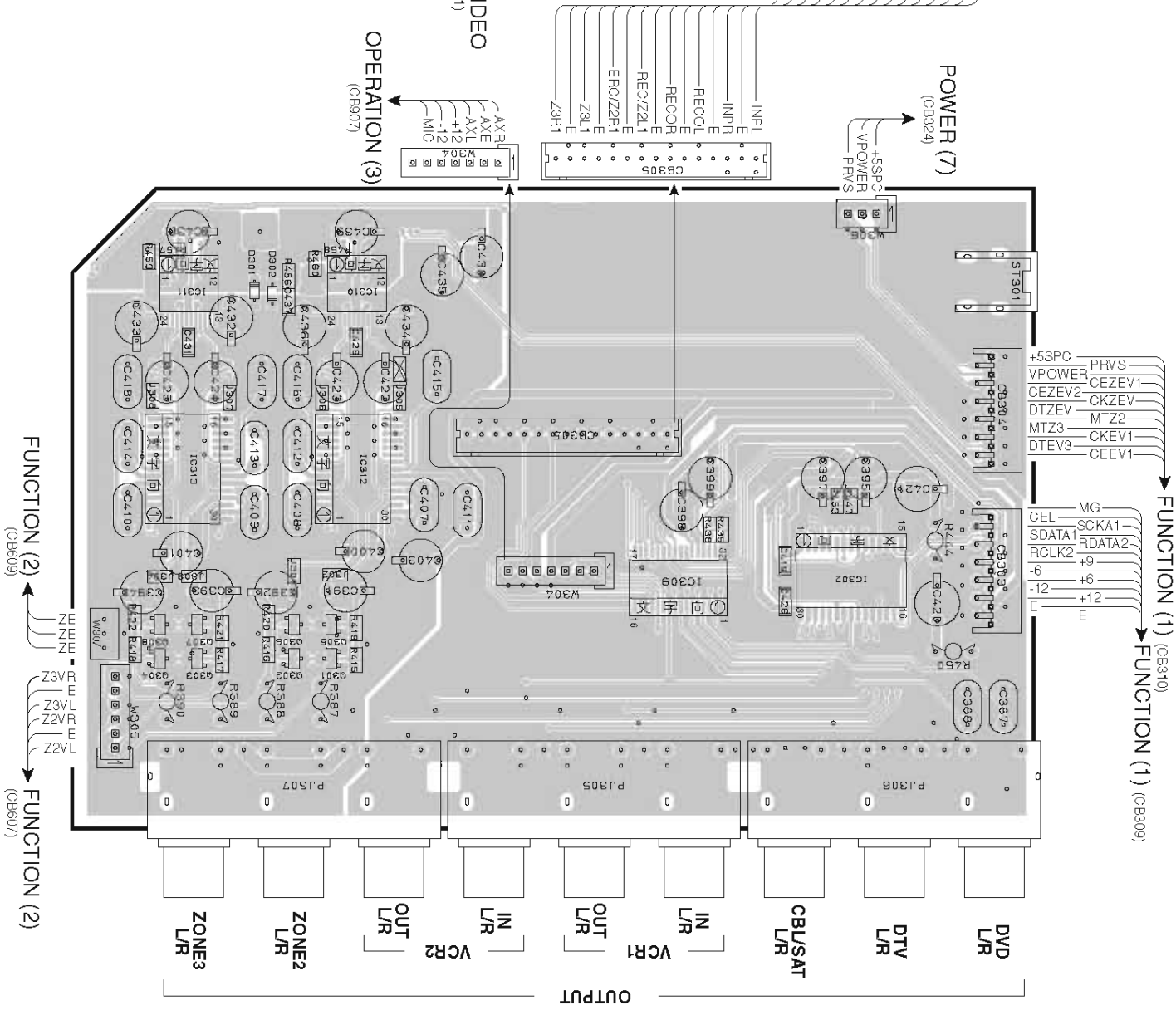
INPUT (2) P.C.B. (Side A) Lead Free Solder Used
