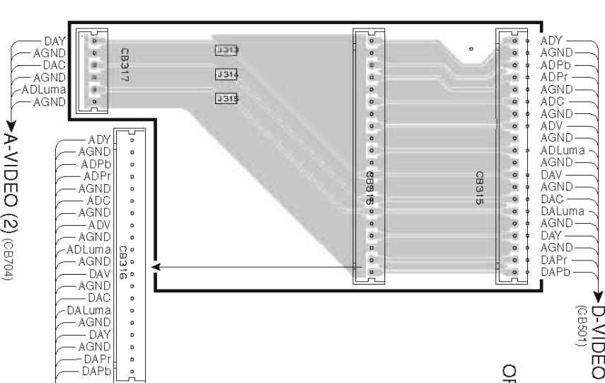
INPUT (5) P.C.B. (Side A) Lead Free Solder Used
