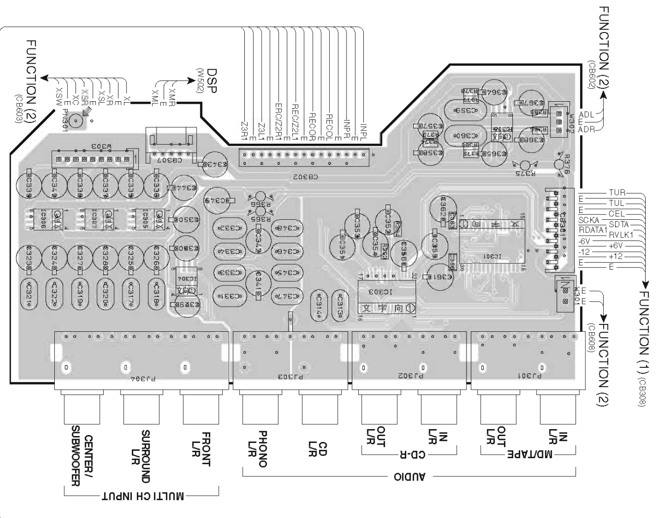
INPUT (5) P.C.B. (Side A) Lead Free Solder Used
