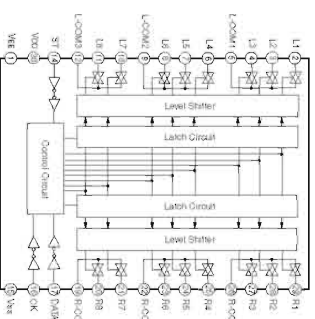
IC301: NJU7912AM Analog function switch
