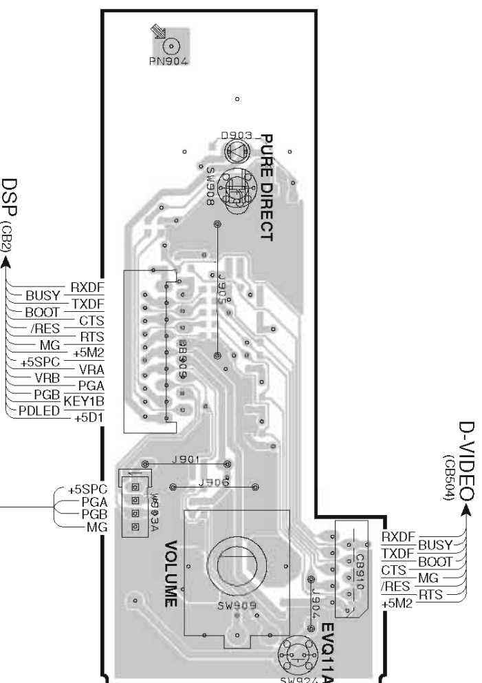
OPERATION (2) P.C.B. (Side A)
