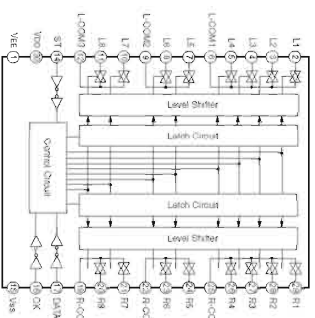
IC302: NJU7913AM Analog function switch
