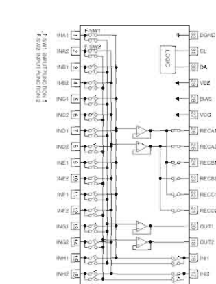
IC303: BD3841FS Function Switch
